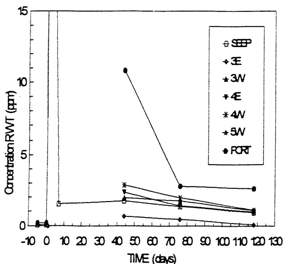
Figure 5 Mine well concentrations of Rhodamine WT with respect to time.
