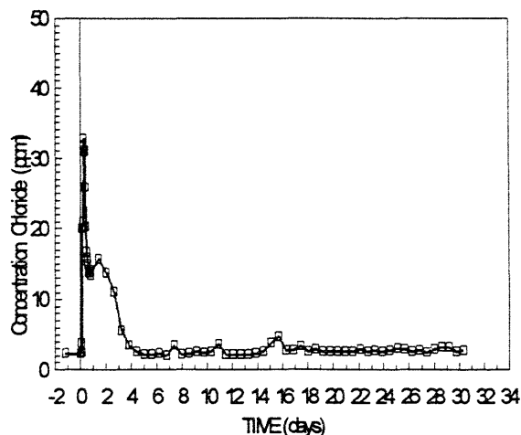
Figure 3 Breakthrough curve of tracer test 2-chloride
