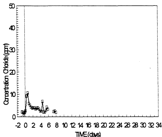
Figure 4 Breakthrough curve of tracer test 3-chloride
